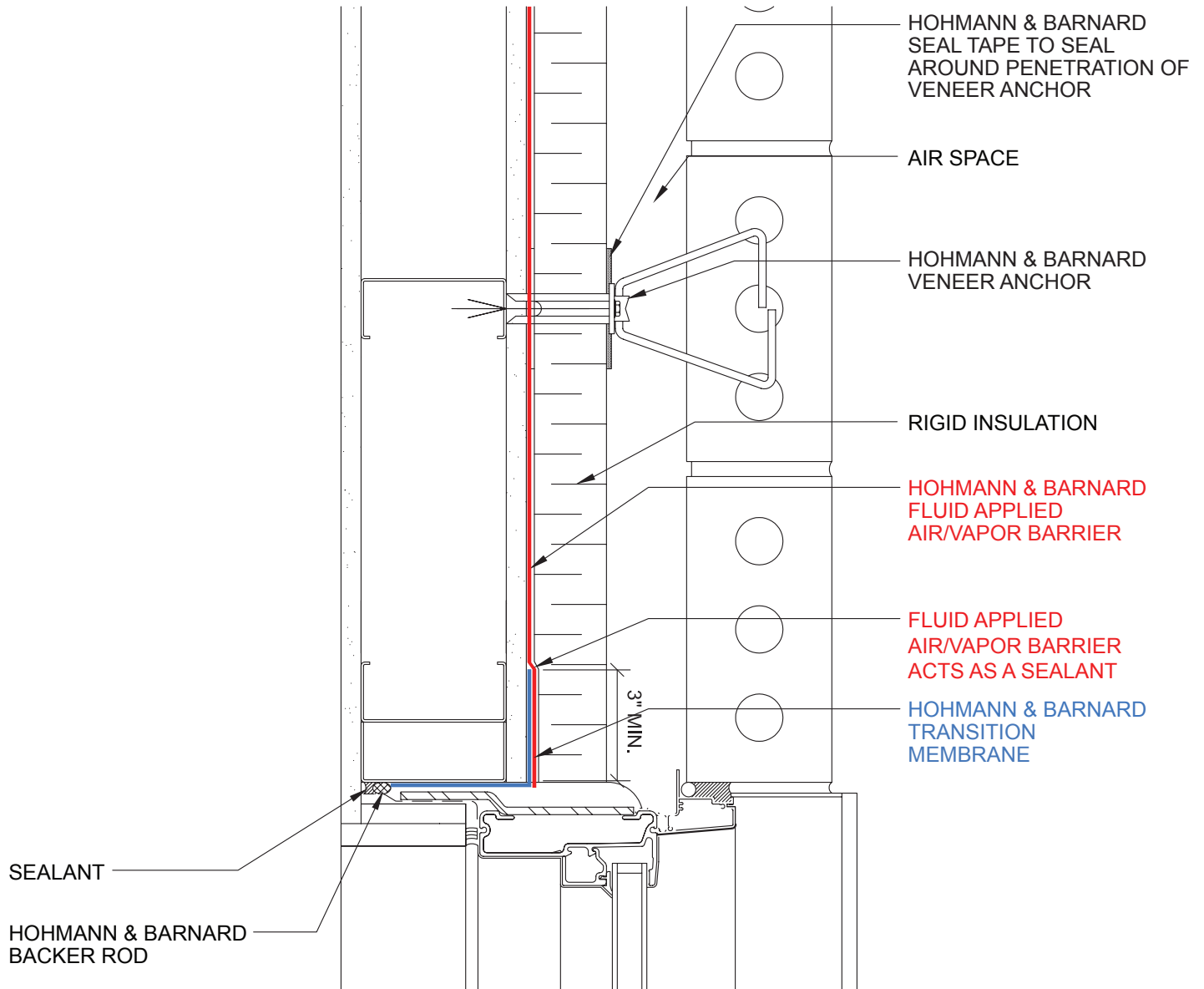
PLAN VIEW
